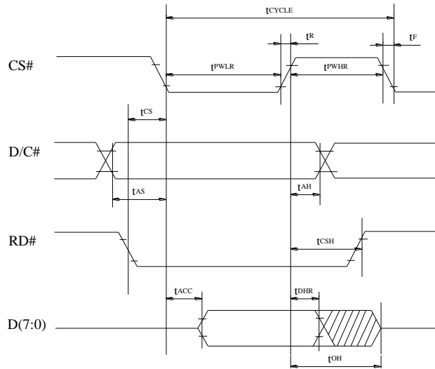
Write cycle(Form 2)
