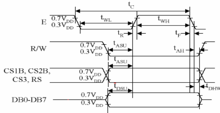
MPU Write Timing
